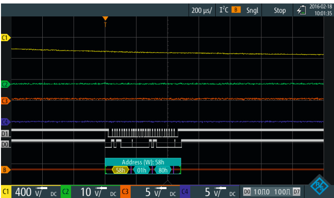
Ramp-up of an embedded AC/DC converter, programmed by PMBus/I 2 C command (C1: 230 V AC input; C2: 12 V DC output; C3: 5 V DC output; C4: power good; D1: I 2 C_SCL; D0: I 2 C_SDA; B: I 2 C bus decoding).
