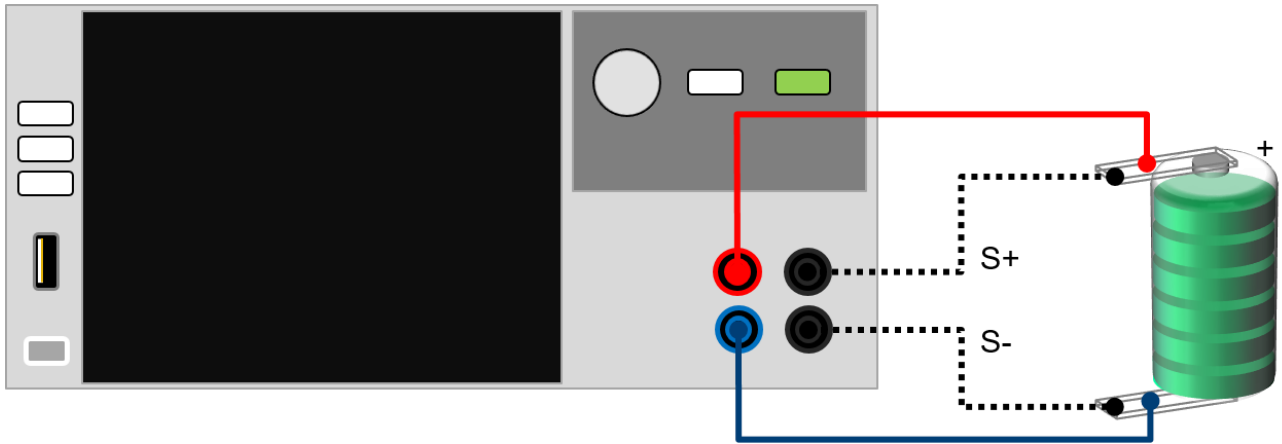
Figure 6: Measurement setup
