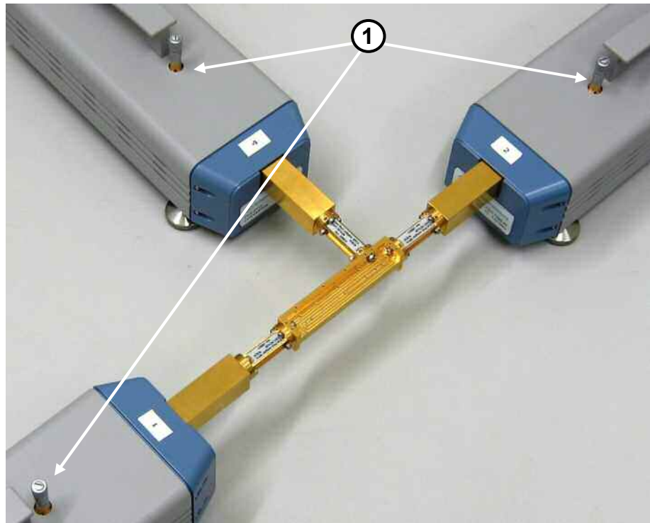
Fig. 4.5: Trial setup for directivity measurement
