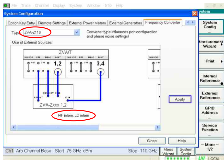
Fig. 4.2: Configuring the converters on the R&S® ZVT20
