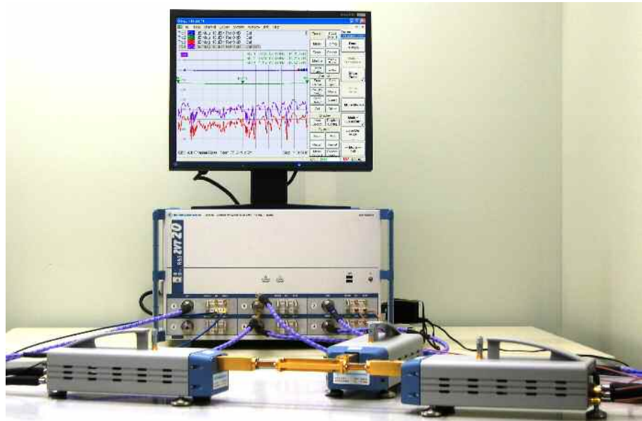
Fig. 4.1: Test setup with DUT
