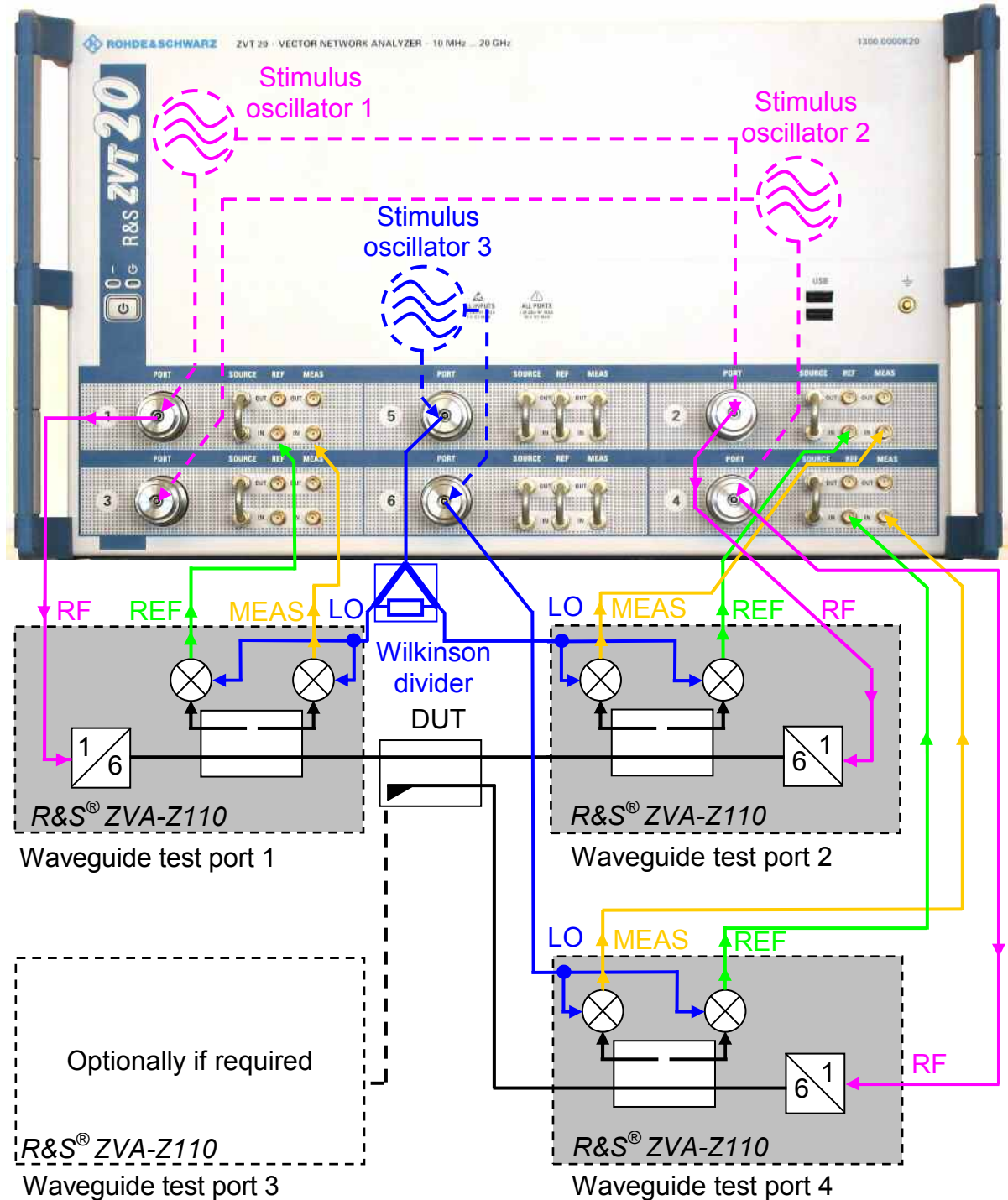
Fig. 4.4: Cabling scheme for three (four) converters and a six-port R&S® ZVT without an external generator
