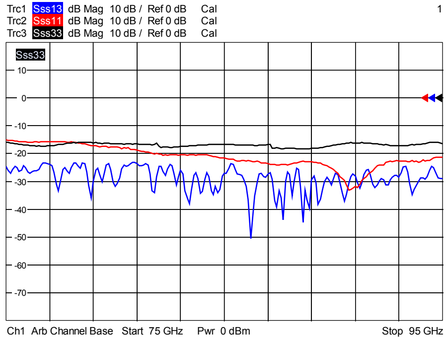
Fig. 4.24: Results of selected unbalanced measurements: isolation between ports 1 and 3, matching at ports 1 and 3
