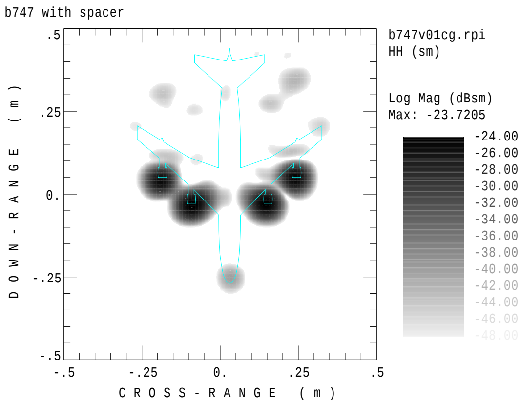
Figure 21: ISAR image of a B747 (1:100 scale).
