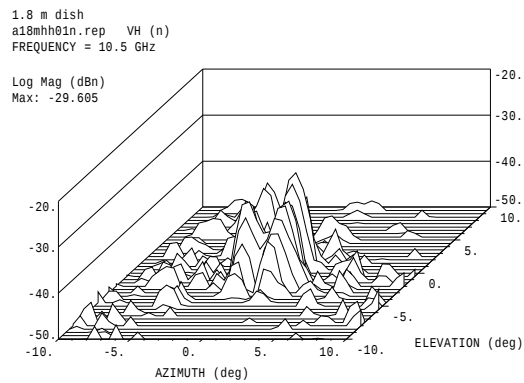
Figure 3b: Cross-polarization pattern at 10.5 GHz.
