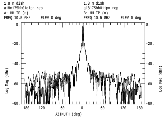
Figure 4b: Cross-polarization pattern at 10.5 GHz. —— gated ----- ungated
