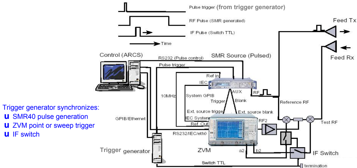
Figure 12: Antenna and RCS measurement system for pulse profile measurements.
