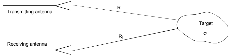
Figure 15: Transmitter, target and receiver geometry for radar range equation.
