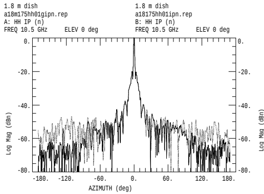
Figure 6a: Co-polarization pattern at 10.5 GHz. —— no mixers ----- fixed IF mode
