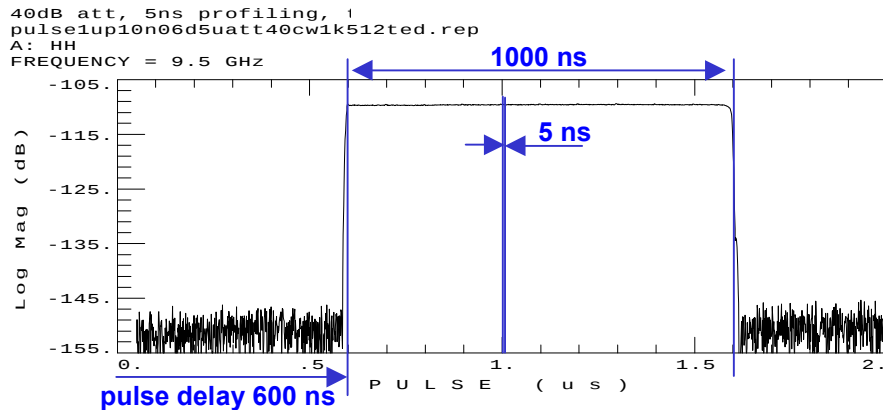
Figure 14: Pulse profile measurement results, derived by external software from the ZVM frequency sweep with quasi zero span.
