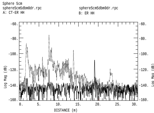
Figure 18: Time domain calibration. - - - - empty chamber (EC) —— Calibration sphere - EC
