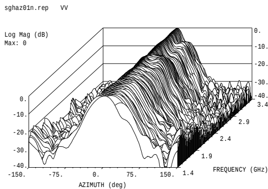
Figure 8: Ungated pattern for 1.4 GHz to -3.4 GHz
