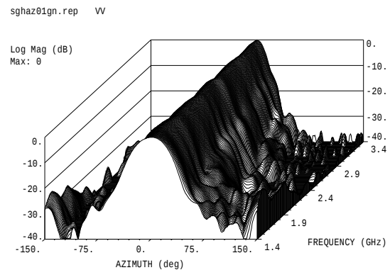
Figure 9: Gated pattern for 1.4 - 3.4 GHz
