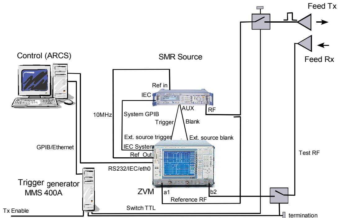
Figure 7: Antenna measurements with pulse generator.
