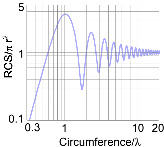
Figure 16: RCS of a metal sphere.
