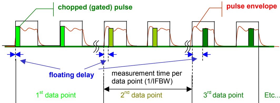
Figure 13: Principle of pulse profile measurement
