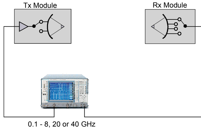
Figure 2: Antenna measurements - basic configuration.
