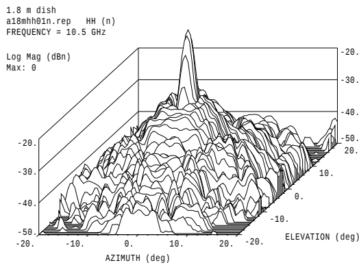
Figure 3a: Co-polarization pattern at 10.5 GHz.
