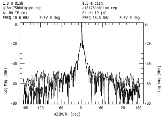
Figure 4a: Co-polarization pattern at 10.5 GHz. —— gated ----- ungated
