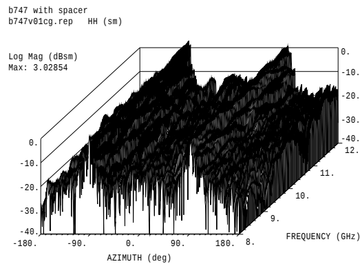
Figure 20: RCS response for \pm 180^\circ and 8-12 GHz.
