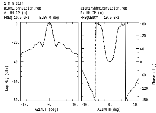
Figure 6b: Cross-polarization and phase pattern at 10.5 GHz. —— no mixers ----- fixed IF mode
